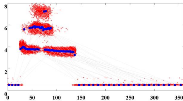
Fig. 12. Dataset and Prototype Vector (Corona Discharge)
