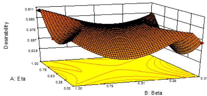
Fig. 19. Desirability plot to optimize multiple responses.
