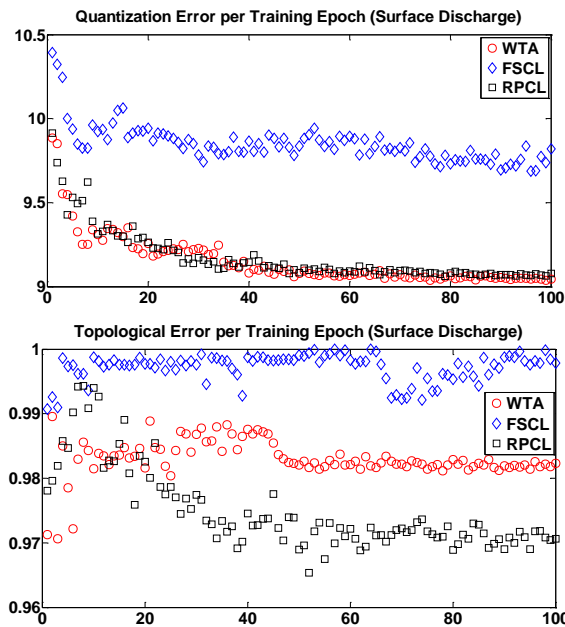
Fig. 7. Quantization and Topological error per Training Epoch (Surface Discharge)
