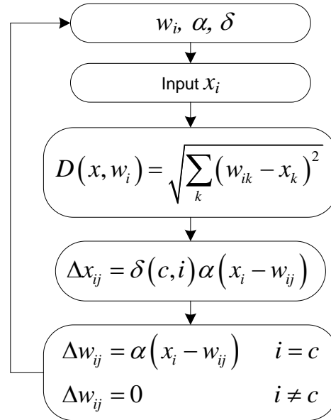
Fig. 5. Flow chart of SOM.
