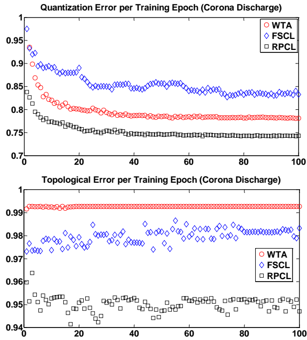
Fig. 9. Quantization and Topological error per Training Epoch (Corona Discharge)
