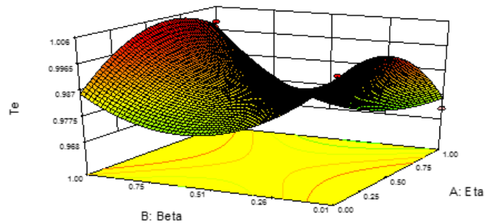
Fig. 17. Surface plot of the combined effects of the te .
