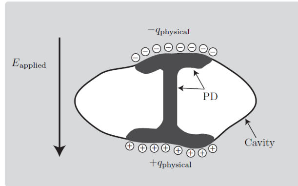
Fig.2. Schematic picture of a partial discharge in a cavity
