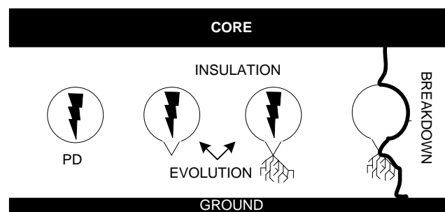
Fig. 1. Example of damage in a polymeric power cable from the PD in a cavity to breakdown.
