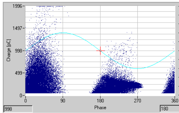
Fig. 3. Example of a partial discharge pattern
