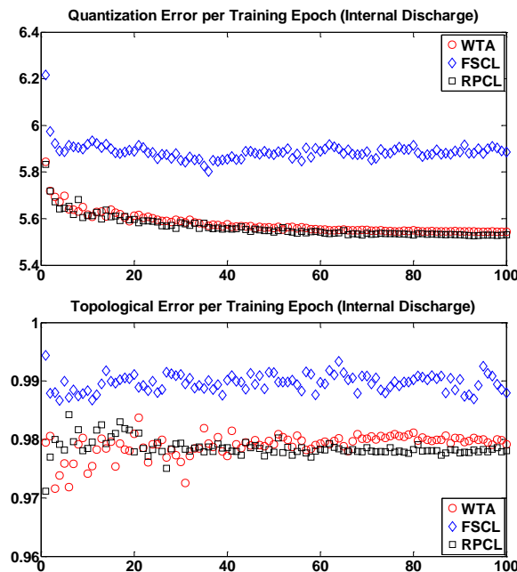
Fig. 8. Quantization and Topological error per Training Epoch (Internal Discharge)
