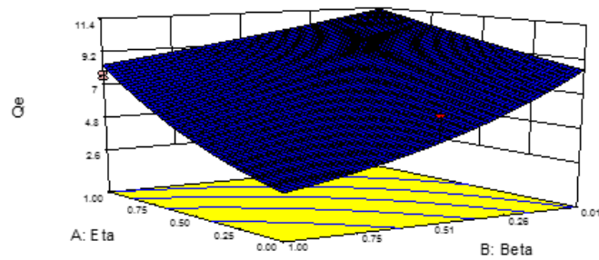
Fig. 16. Surface plot of the combined effects of the qe .
